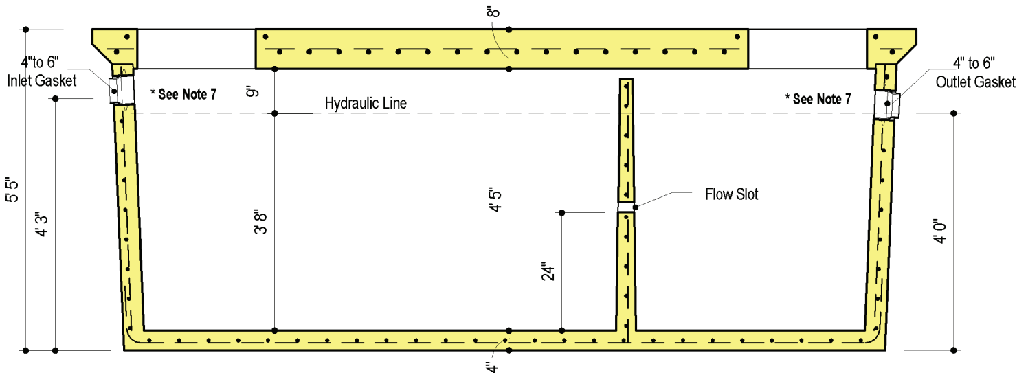
SECTION VIEW
