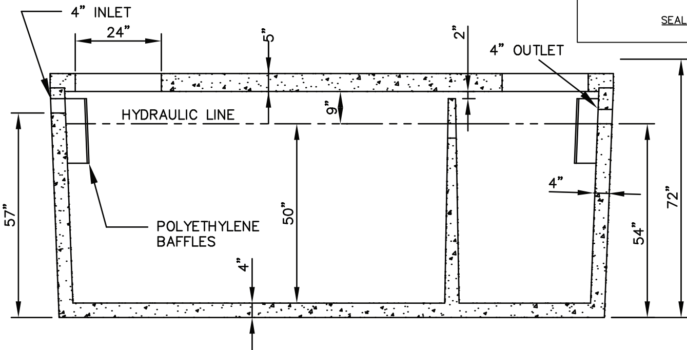
SECTION VIEW
