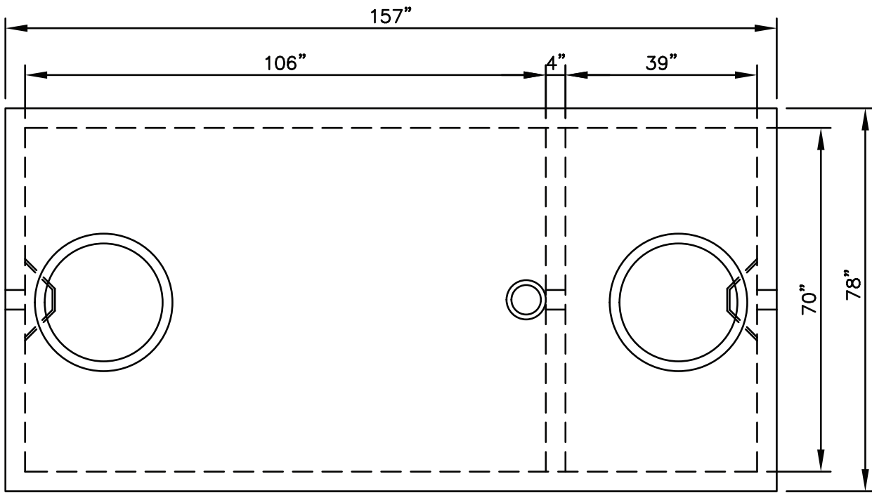
PLAN VIEW
