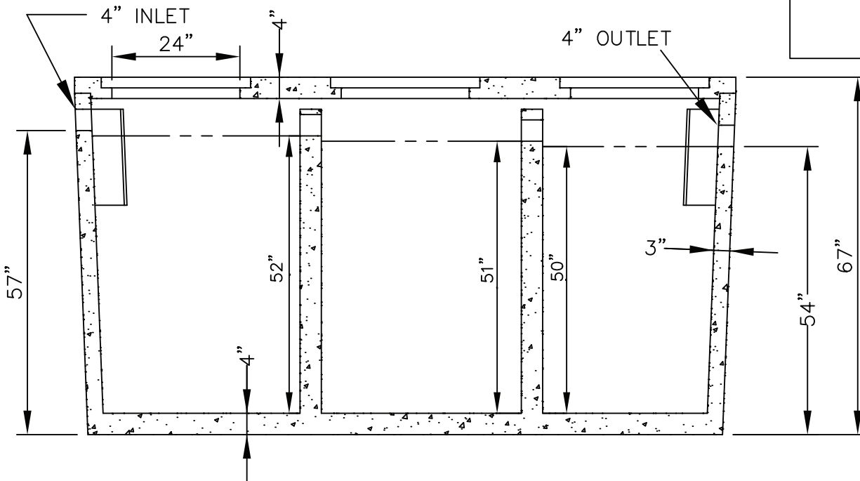
SECTION VIEW
