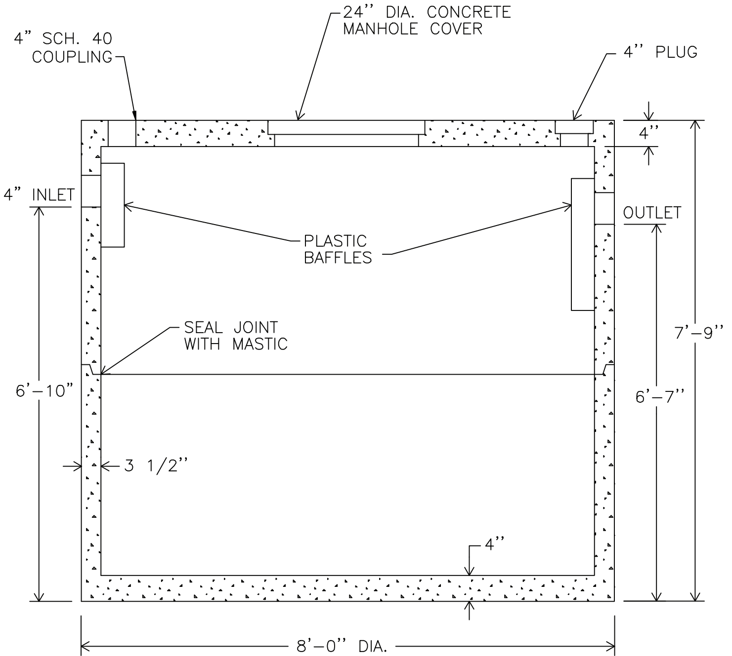
—SECTION ELEVATION—
