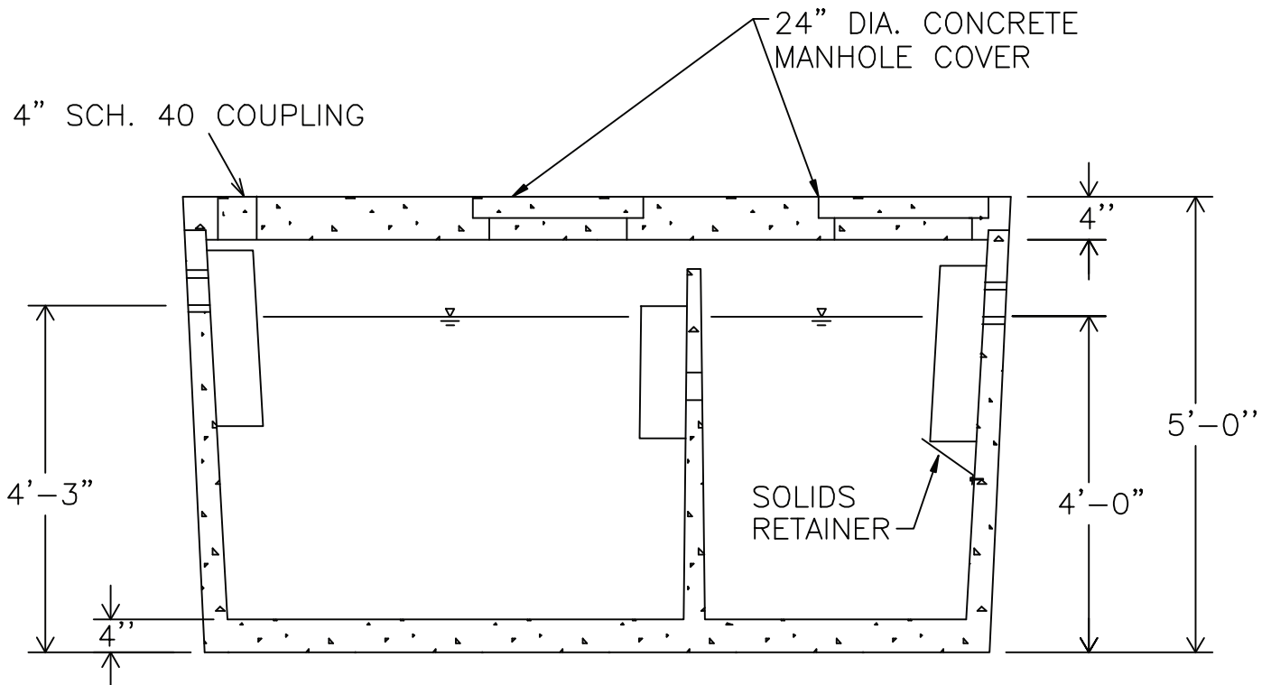
—SECTION—
