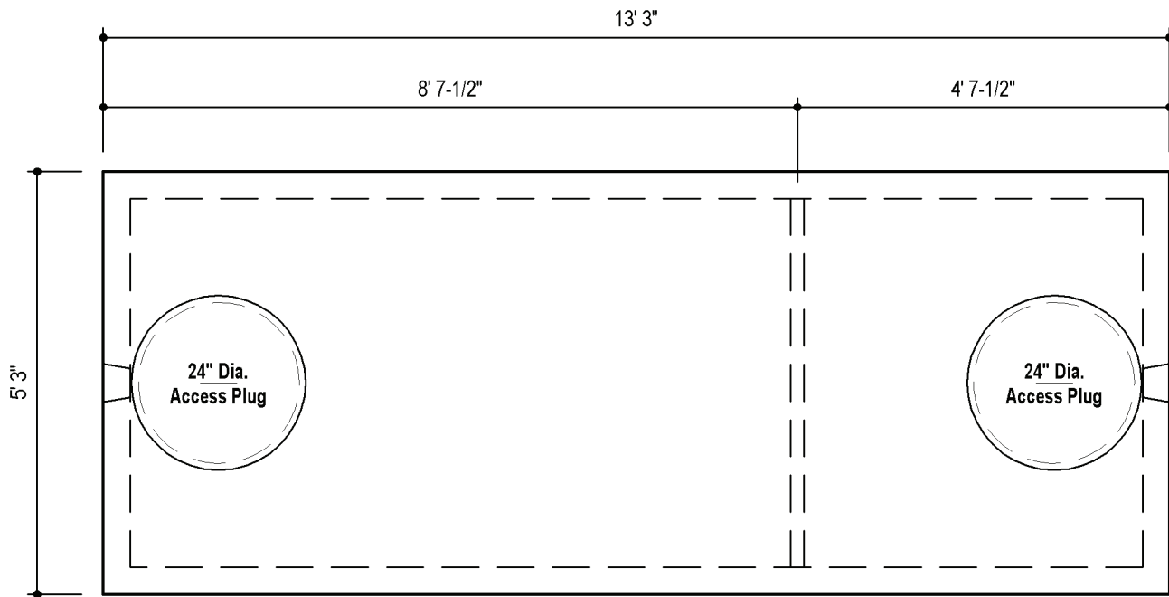
PLAN VIEW
