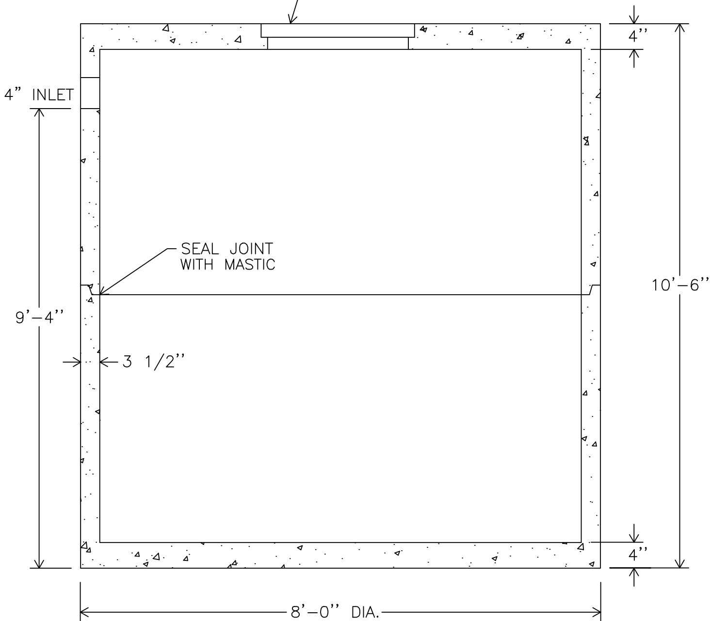
-SECTION ELEVATION-
