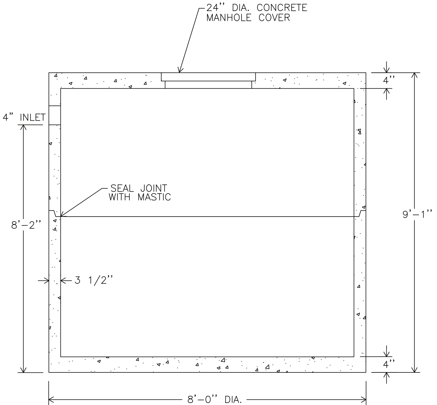
-SECTION ELEVATION-
